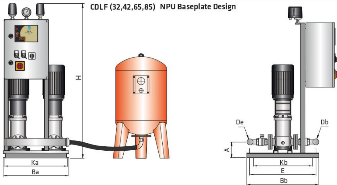
CDLF (32,42,65,85) NPU Baseplate Design
